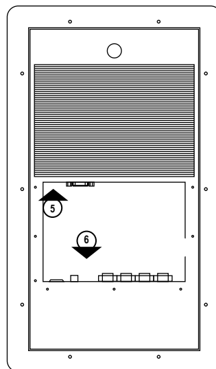
2 INTERCOM BACK ELEVATION NOT TO SCALE
