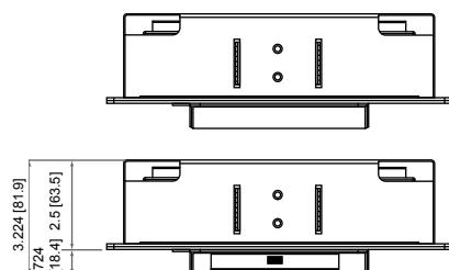
4 INTERCOM TOP/BOTTOM VIEWS NOT TO SCALE
