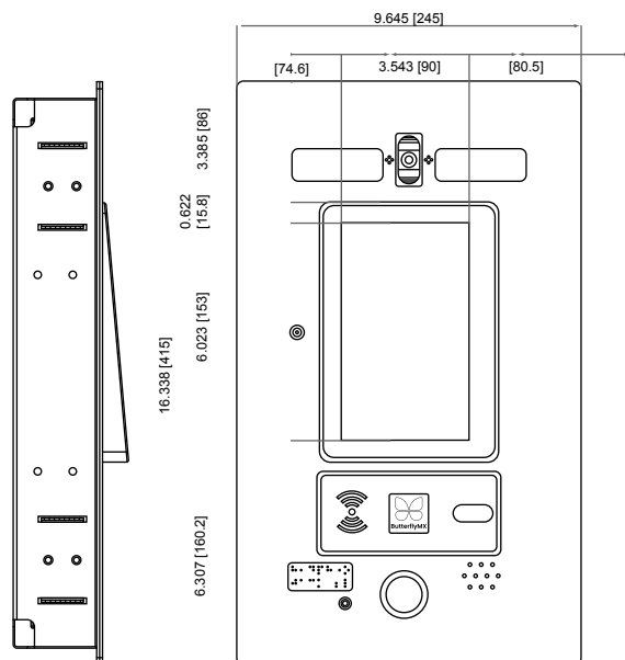
1 INTERCOM FRONT ELEVATION NOT TO SCALE
