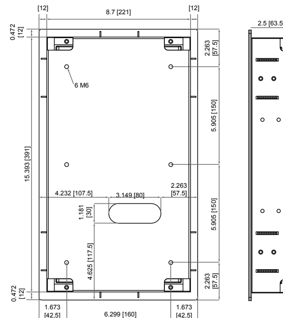
3 BACKBOX REAR AND SIDE ELEVATION NOT TO SCALE
