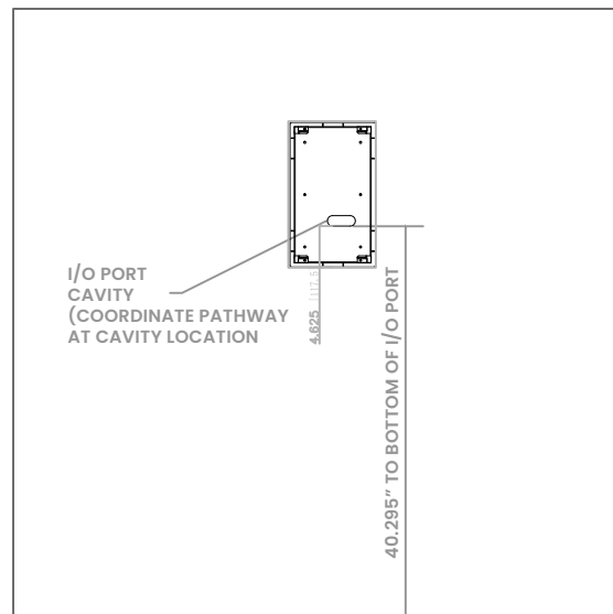
2 FRONT VIEW: BACKBOX PLACEMENT NOT TO SCALE
