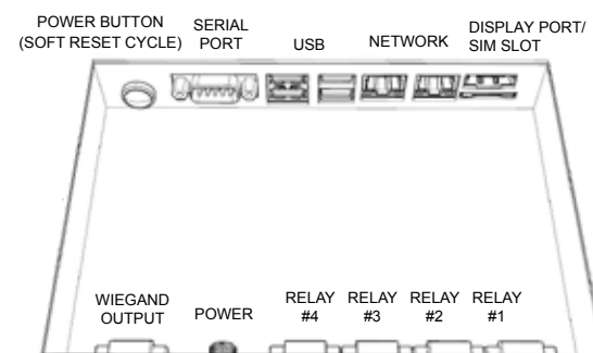
5 I/O PORT DETAIL NOT TO SCALE
