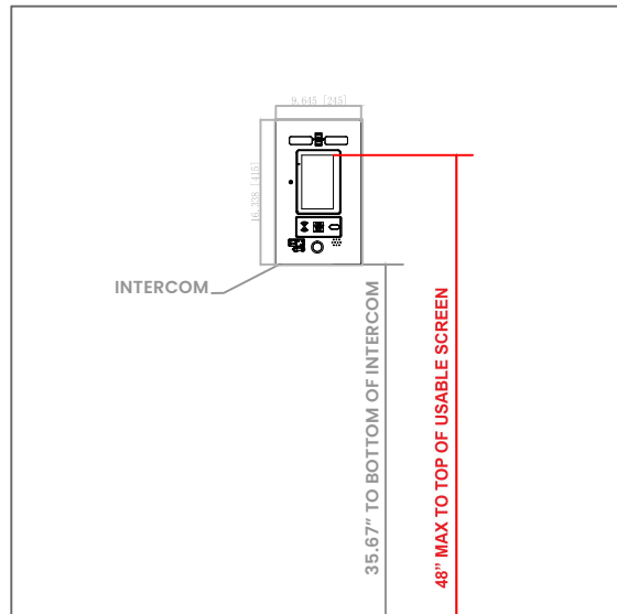
1 FRONT VIEW NOT TO SCALE
